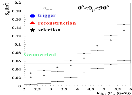
Figure 2. Effective area as a function of simulated upward-going muon energy.
