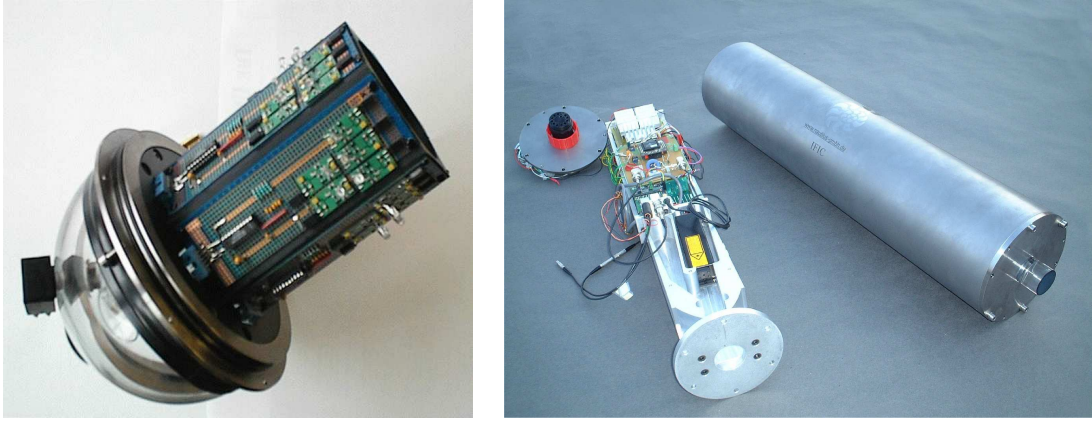
Fig. 1. Left: internal mounting of an LED beacon holding the 6 LED faces. Right: blow-up of a laser beacon. The internal electronics, the laser and the external titanium container with the quartz rod on its upper surface can be seen.
