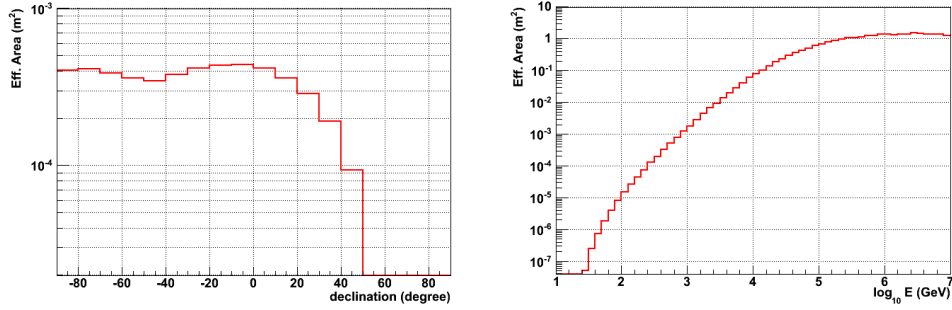
Figure 5.16: Effective area as a function of the true neutrino declination (left) and true neutrino energy (right) for the optimal cuts.
