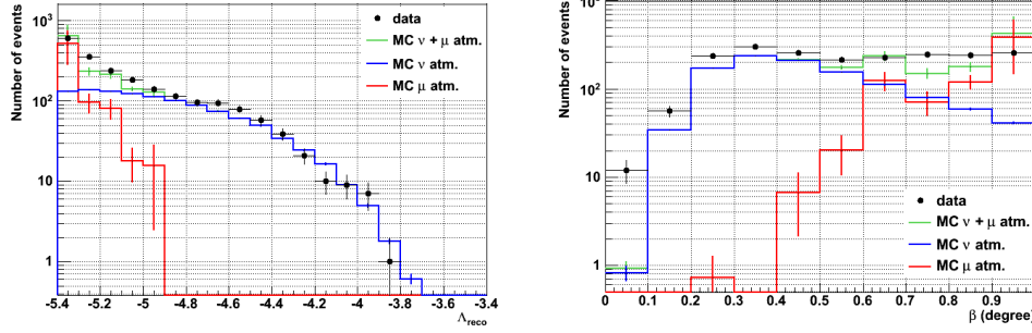
Figure 6.1: Distributions of \Lambda_{\text{reco}} (left) and \beta (right) of the data and Monte-Carlo for the optimized cuts.
