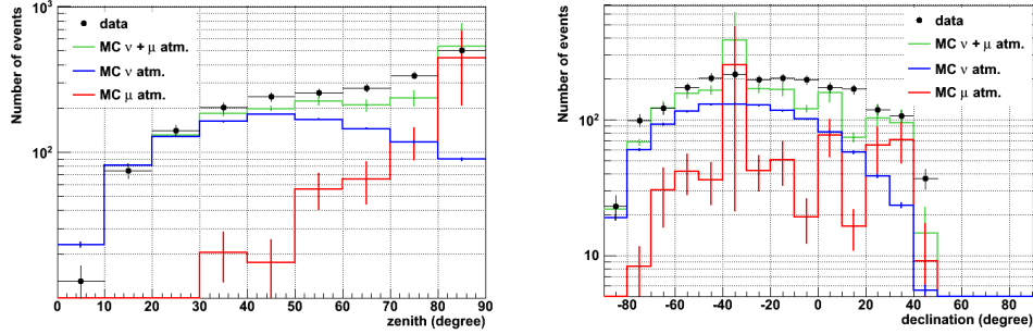
Figure 6.2: Zenith (left) and declination (right) distributions of the data and the Monte-Carlo for the optimized cuts.
