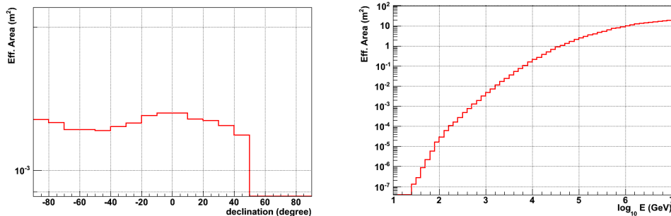
Figure 6.3: The effective area as a function of the true neutrino declination (left) and the true neutrino energy (right).
